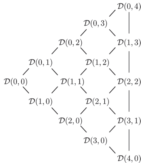
Fig. 1. The Hasse diagram of P for r = 4
